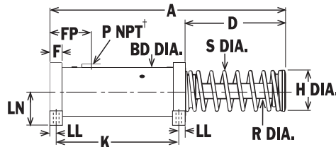
RECTANGULAR FLANGE
